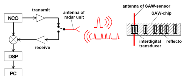
Fig. 2 Working principle of the high-frequency temperature measuring system based on wireless passive SAW temperature sensors (NCO = Numeric Controlled Oscillator, DSP = Digital Signal Processor, PC = Personal Computer) [1]
