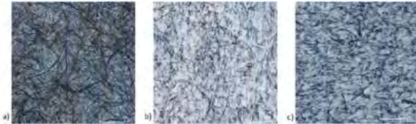
Figure 1 a) The standard Burnout-Test [3] applied to a TMP handsheet. The fibers are not sufficiently blackened. b) Standard Burnout test [3], wood fibers carbonized incompletely. c) Result of the new Burnout Test, all fibers are entirely and evenly blackened.
