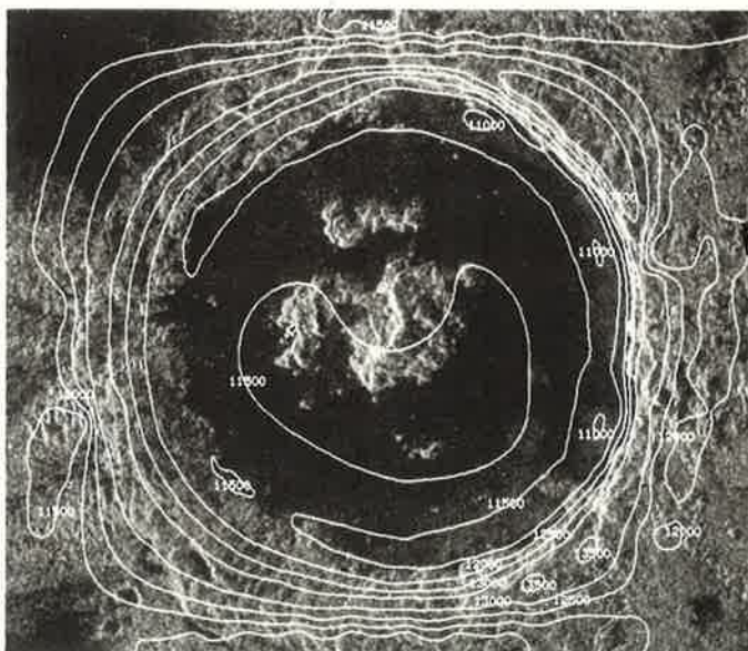
FIG. 14. Contour plot produced from the DEM created from the symmetry method, at 500-metre intervals. The DEM is a combination of the standard GTDR-altimetry DEM and the symmetry method and presents a rim height of 1,500 metres above the floor, and a slope of 21°.
