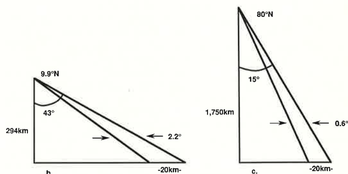
FIG. 11. Approximate look angles off nadir, and variation of look angles within the imaged swath. (a) General graph; (b) At periaapsis; (c) At 80° North. Any overlapping images will have differences in incidence angles that are smaller than look angle variations within one swath.
