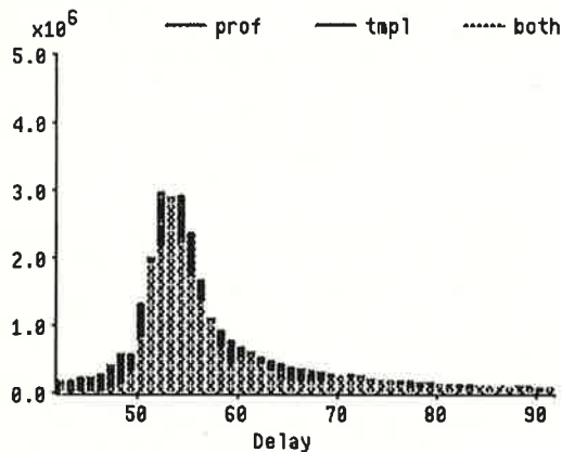
FIG. 5. Individual altimeter trace or echo function from footprint A (see Figure 4). The difficulty exists in allocating the strongest echo (the peak) to a specific location within the footprint. Image produced with the MGNDQE Software (Courtesy P. Ford, MIT).
