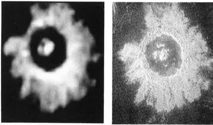
(a) Arecibo Image
