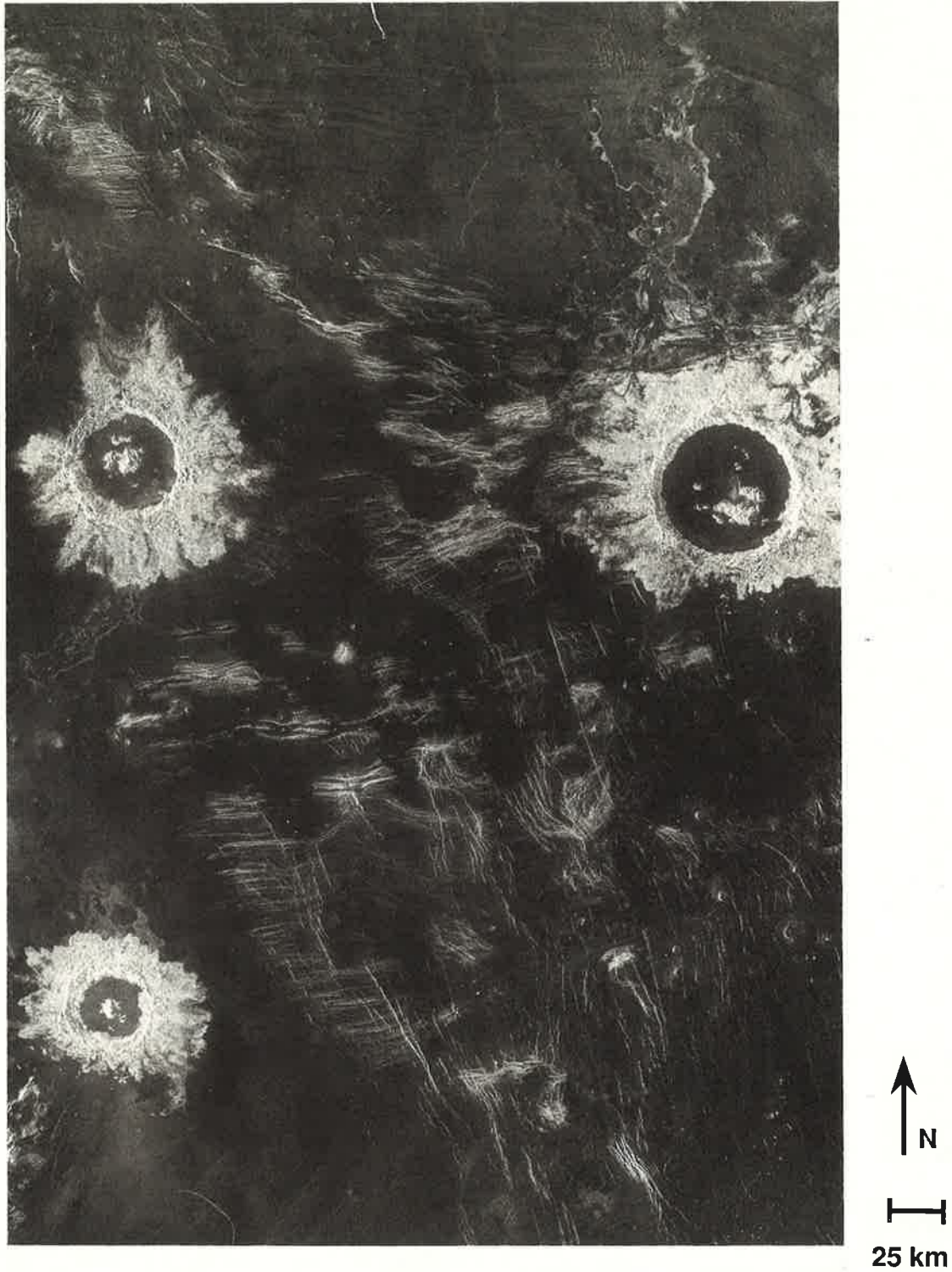
FIG. 1. Mosaicked imaging product of the crater farm at 27°S, 339°E. This is a partial F-MDR covering a width of 300 km and consisting of 23 orbits. At 8 pixels per millimetre, this lends itself for presentation at a Scale 1: 600,000. The northwestern-most crater (above left) is Danilova and subject to analysis in this report.
