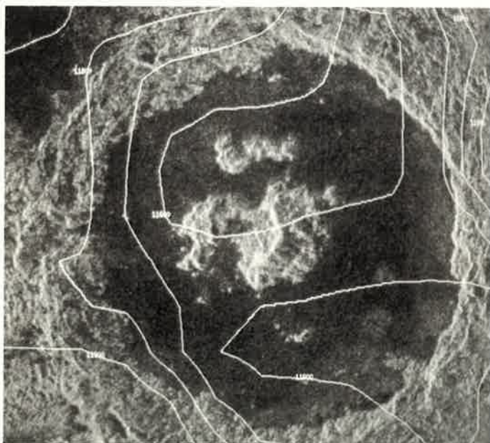
FIG. 12. Contour plot at 100 metres over Crater Danilova, obtained from the standard GTDR-altimetry DEM. Note the lack of correspondence between the contour lines and the apparent terrain shape and the elevation differences of about 200 metres between rim and floor.
