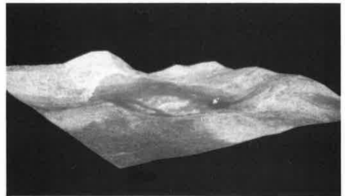
(b) DEM with image overlay
