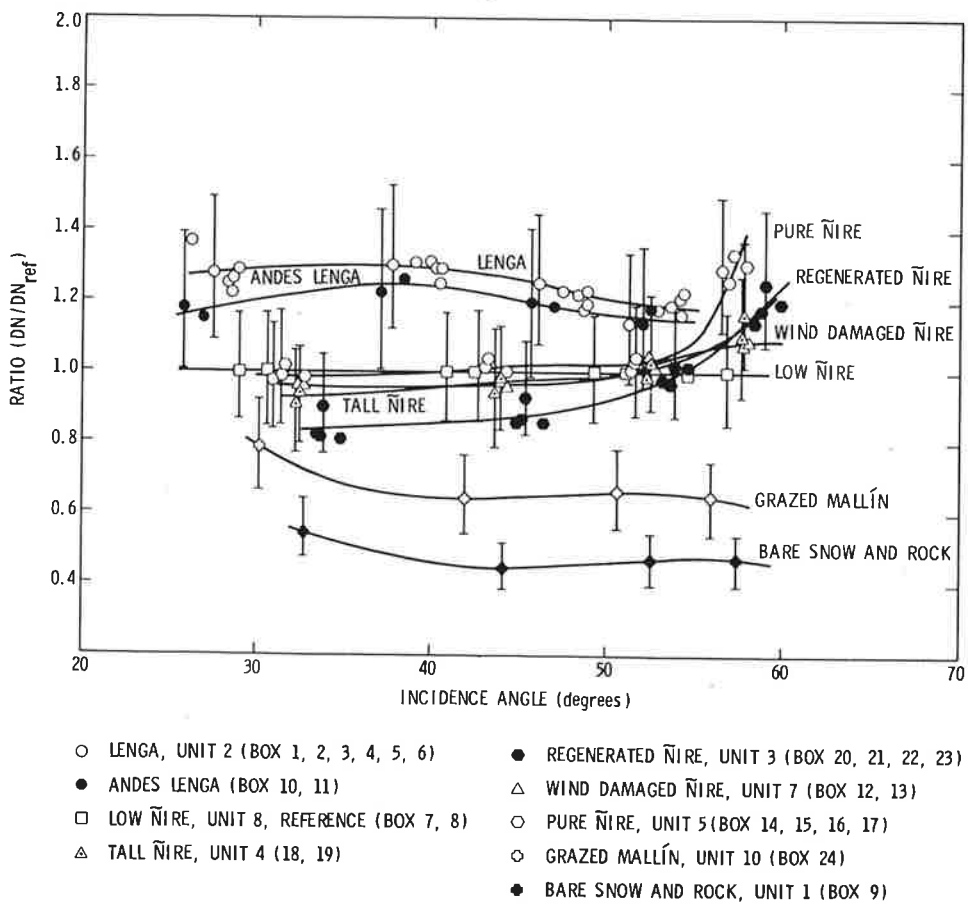
Figure 3. (a) SIR-B image showing location of areas used to generate relative brightness curves; (b) Relative brightness as a function of local incidence angle.
