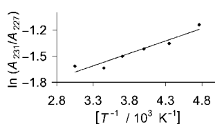
Figure 5. van't Hoff plot for the 231/227 cm -1 band pair of Ge 6 Me 12 in thf solution.
