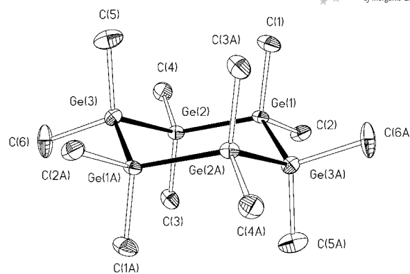
Figure 2. ORTEP plot (30% probability) of the molecular structure of Ge 6 Me 12 , including numbering of the atoms. Hydrogen atoms have been omitted for clarity. Selected bond lengths [Å] and bond angles [°] (with standard deviations): Ge(1)–Ge(2) 2.4094(19), Ge(1)–Ge(3A) 2.4242(17), Ge(2)–Ge(3) 2.4300(16), Ge(1)–C(1) 1.971(11), Ge(1)–C(2) 1.979(11), Ge(2)–C(3) 1.994(11), Ge(2)–C(4) 1.969(11), Ge(3)–C(5) 1.987(11), Ge(3)–C(6) 1.982(13), Ge(1)–Ge(2)–Ge(3) 111.13(6), Ge(2)–Ge(3)–Ge(1A) 111.56(6), Ge(2)–Ge(1)–Ge(3A) 113.32(6), C(1)–Ge(1)–Ge(2) 109.0(4), C(1)–Ge(1)–Ge(3A) 106.7(4), C(1)–Ge(1)–C(2) 108.4(5), C(1)–Ge(1)–Ge(2)–Ge(3) –65.2(4), C(2)–Ge(1)–Ge(2)–Ge(3) 177.0(3), Ge(3A)–Ge(1)–Ge(2)–Ge(3) 53.45(8), Ge(1)–Ge(2)–Ge(3)–Ge(1A) –52.49(8).
