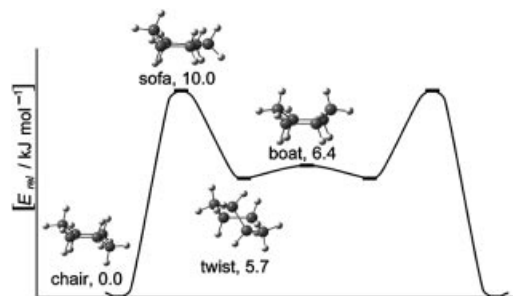
Figure 1. Calculated minima and transition structures of Ge 6 H 12 at the B3LYP/aug-cc-pVTZ level of theory. All relative energies are ZPVE-corrected.
