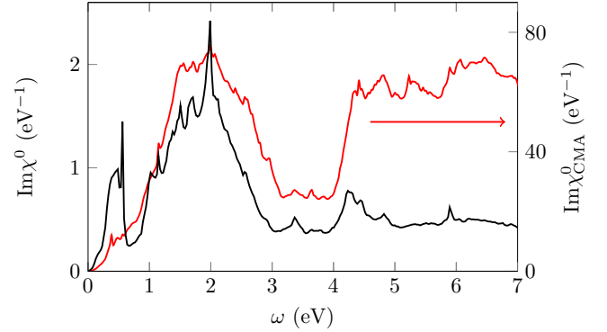
FIG. 9. (Color online) Imaginary part of the dynamic bare susceptibility \chi^0 for FeSe halfway between \Gamma and M. The black line represents the result obtained with exact matrix elements and the red line depicts the CMA result.
