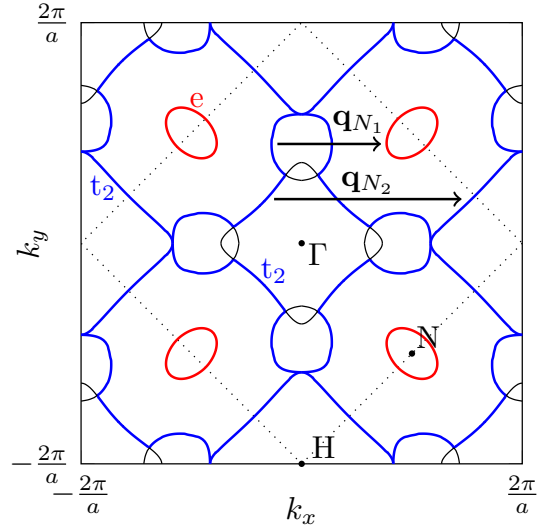
FIG. 3. (Color online) FS of Cr in the k_z=0 plane. The different colors indicate different orbital character as described in Fig. 2 and the boundary of the 1BZ is indicated by dotted lines.
