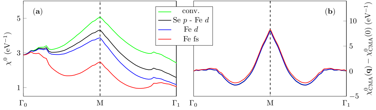
FIG. 7. (Color online) Static bare susceptibility \chi^0 for FeSe at ambient pressure calculated by including different sets of bands, as explained in Fig. 6. The left panel (a) shows the exact result while the right panel (b) contains the CMA result.
