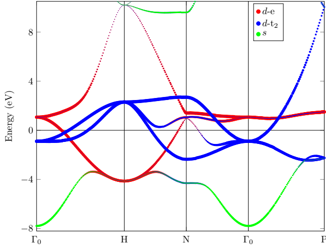
FIG. 2. (Color online) LDA bandstructure of Cr, decorated with partial characters: s (green), d - t_2 (blue), and d - e (red). The coordinates of the high-symmetry points are \Gamma_0=(0,0,0) , H=(0,1,0) , N=(\frac{1}{2},\frac{1}{2},0) , and P=(\frac{1}{2},\frac{1}{2},\frac{1}{2}) , all in units of \frac{2\pi}{a} with a being the lattice constant.
