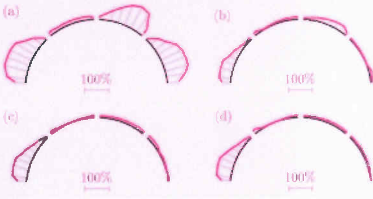
Fig. 11 Semmering pilot tunnel: distribution of the level of loading for (a) t = 12 hours, (b) t = 36 hours, (c) t = 7 days, and (d) t = 9 days.
