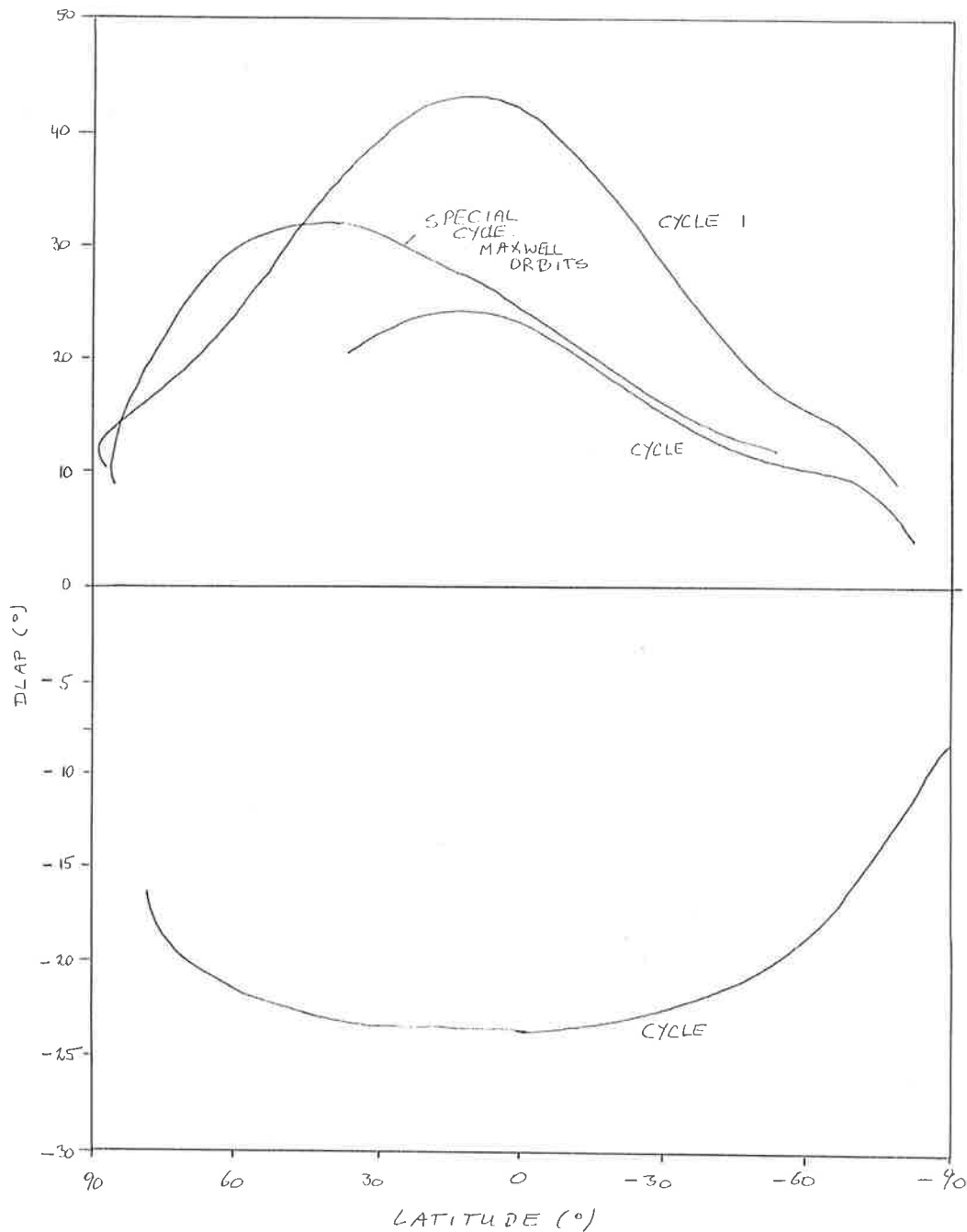
Figure 1: Look-angle profiles during the three initial imaging cycles of Magellan.
