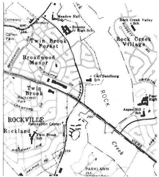
FIG. 1. Segment of an original color separate of a U.S. Geological Survey 1:24,000 scale map (Kensington and Rockville, Maryland) (reduced to 1:32,000 scale).
