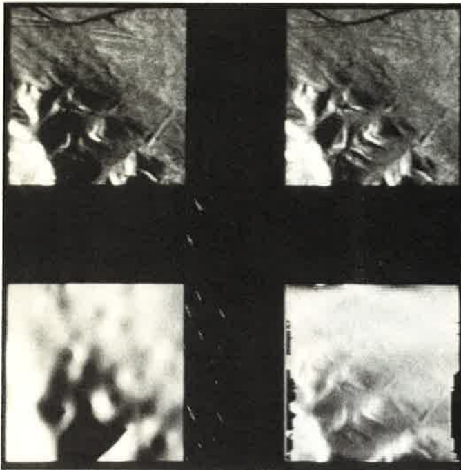
FIG. 16. Test of shape-from-shading over Baffin Island. (Top row - input radar images. Bottom row - illuminated radar stereo height model (left) and illuminated radar shape-from-shading model (right).) Area is 3km by 3km, imaged with STAR-2 of Intera Technologies Ltd., Calgary, Canada, at x-band, 6-m resolution, seven looks. Incidence angles of the input images are 51^\circ and 70^\circ .
