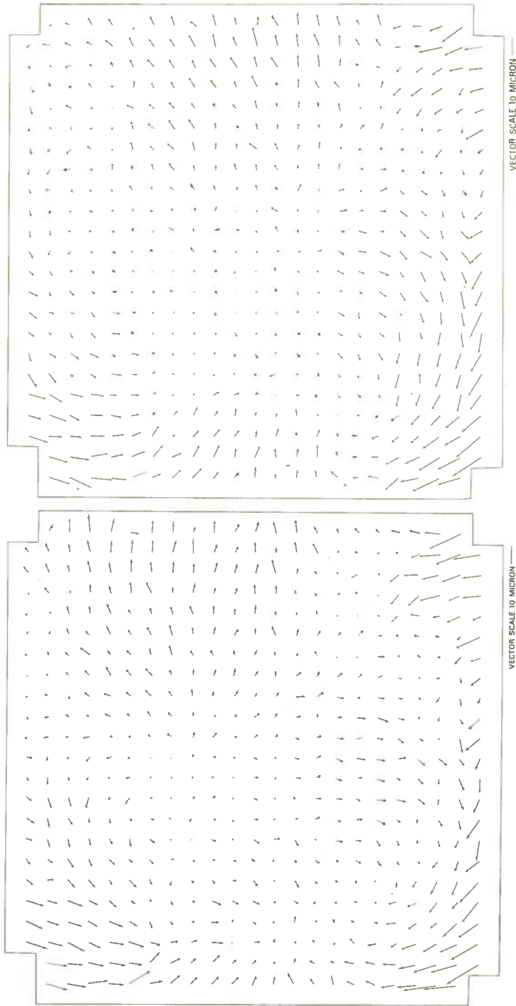
Figure 1 - Residual distortion-plate 302
