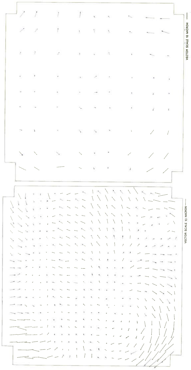
Figure 3 — Residual distortion-plate 412
